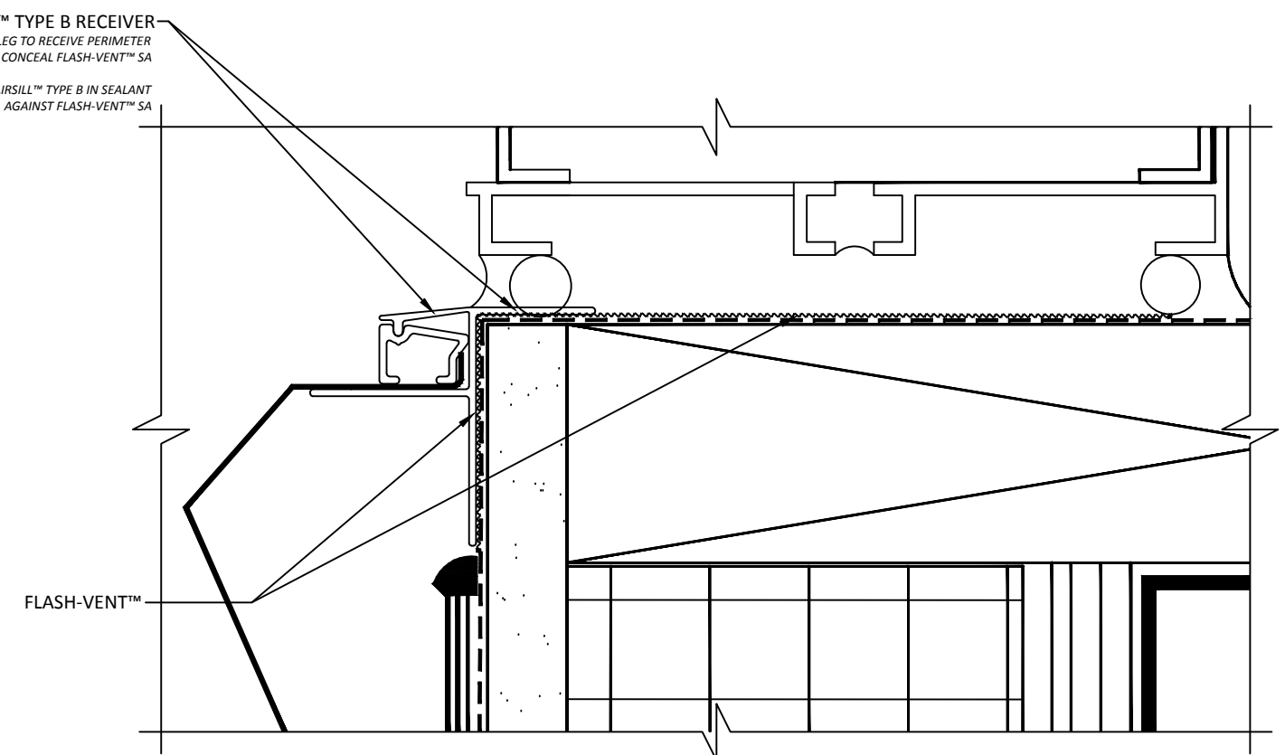
ALTERNATE SILL OPTION - INCORPERATES YORK FLASH-VENT™
