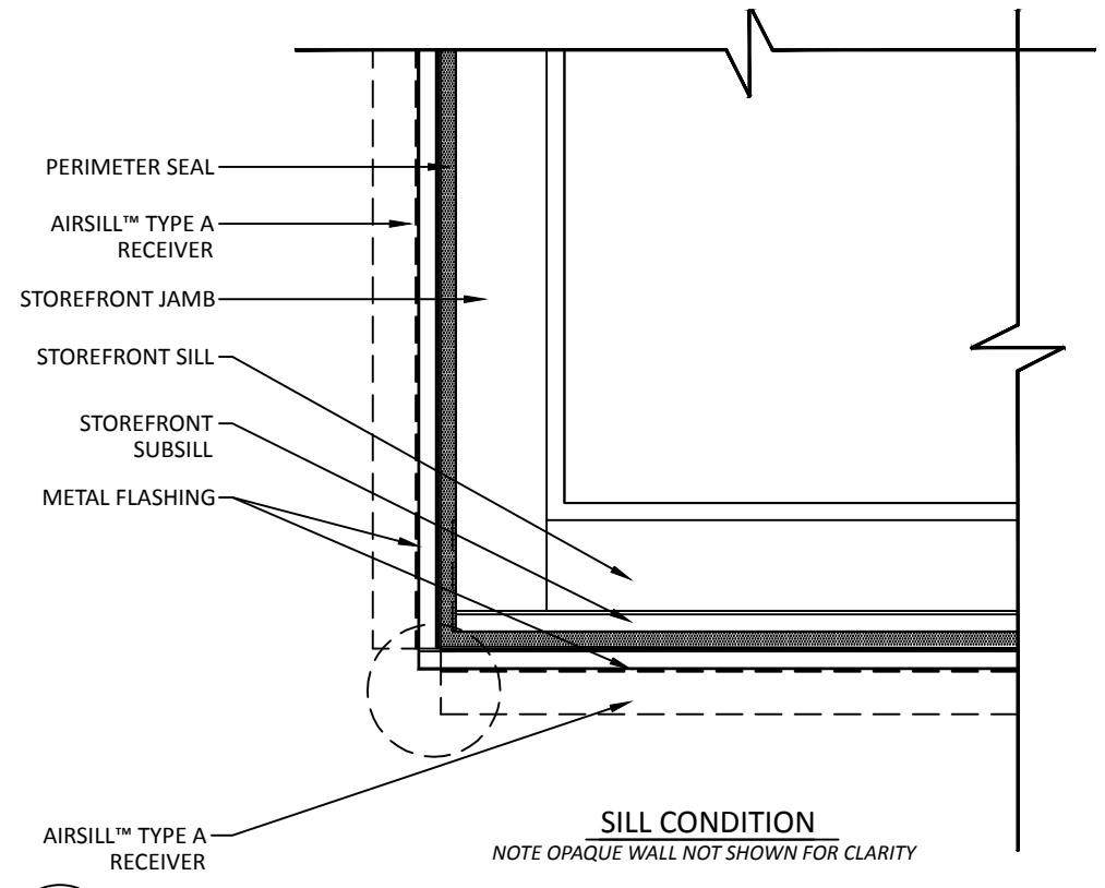
2 AIRSILL™ TYPE A - PERIMETER OPTION
