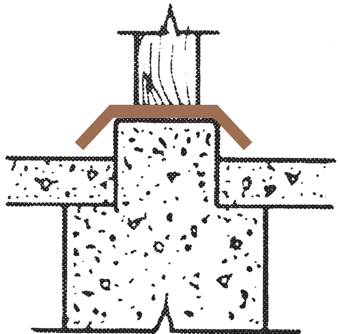
Basement Post
