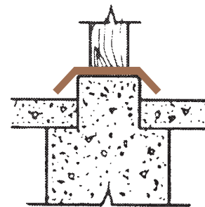
Basement Post
