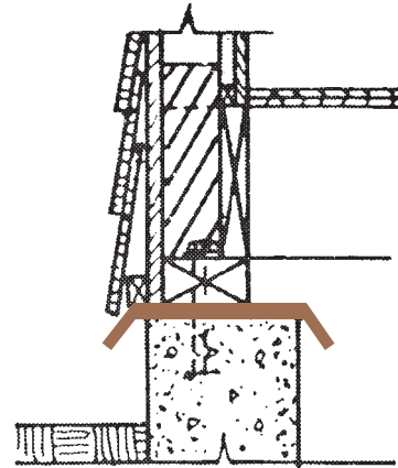
Foundation
