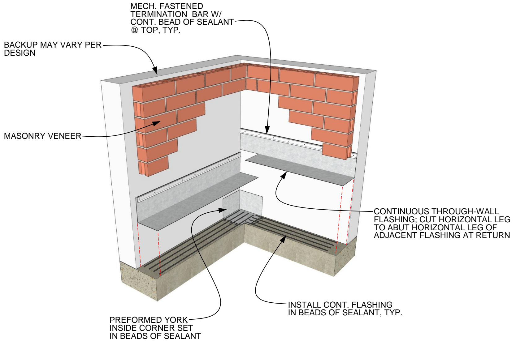
INSIDE CORNER, EXPLODED VIEW YORK® FLASHING DRAWING NO. 03-02 REV. 3/29/14
