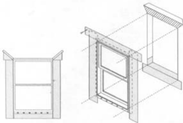
Flanged Window Flashing Installation AFTER Weather-Resistive Barrier
