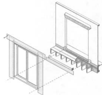
Exterior Sliding Door with Deck
