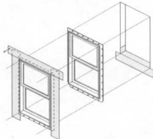
Flanged Window Flashing Installation BEFORE Weather-Resistive Barrier Option 1 – Low Exposure
